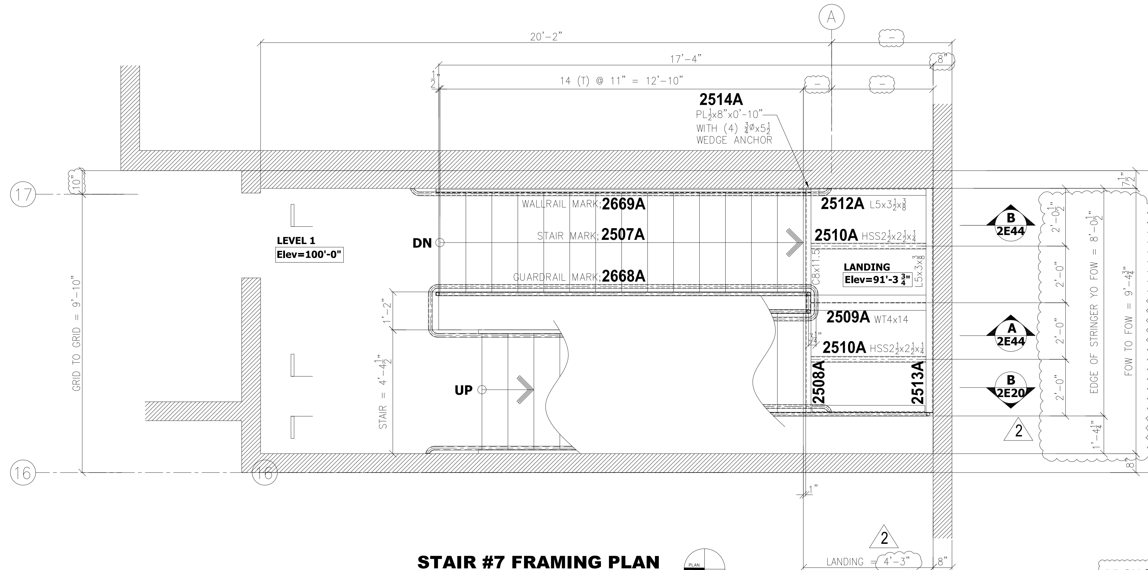
STAIR #7 FRAMING PLAN LEVEL 1
