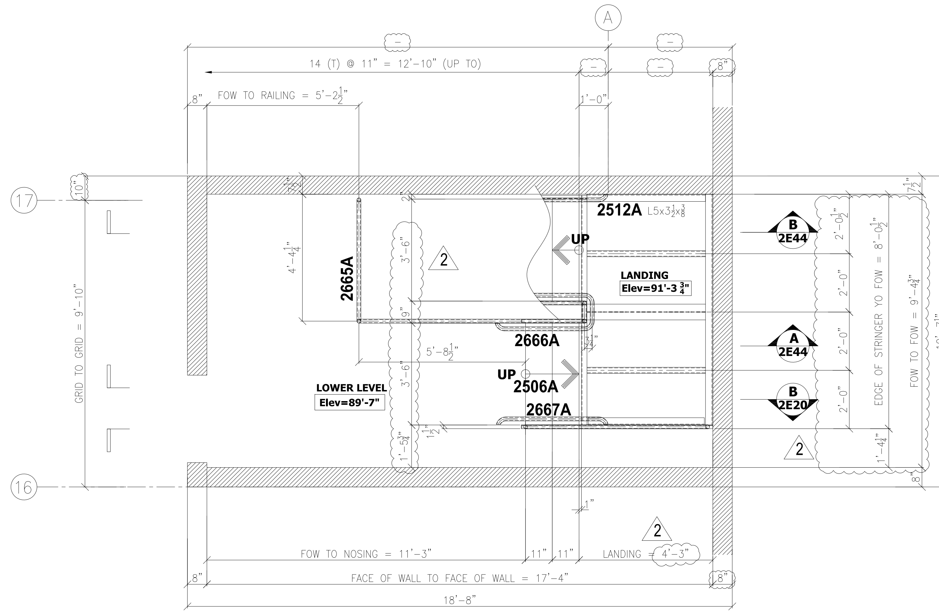
STAIR #7 FRAMING PLAN LOWER LEVEL
